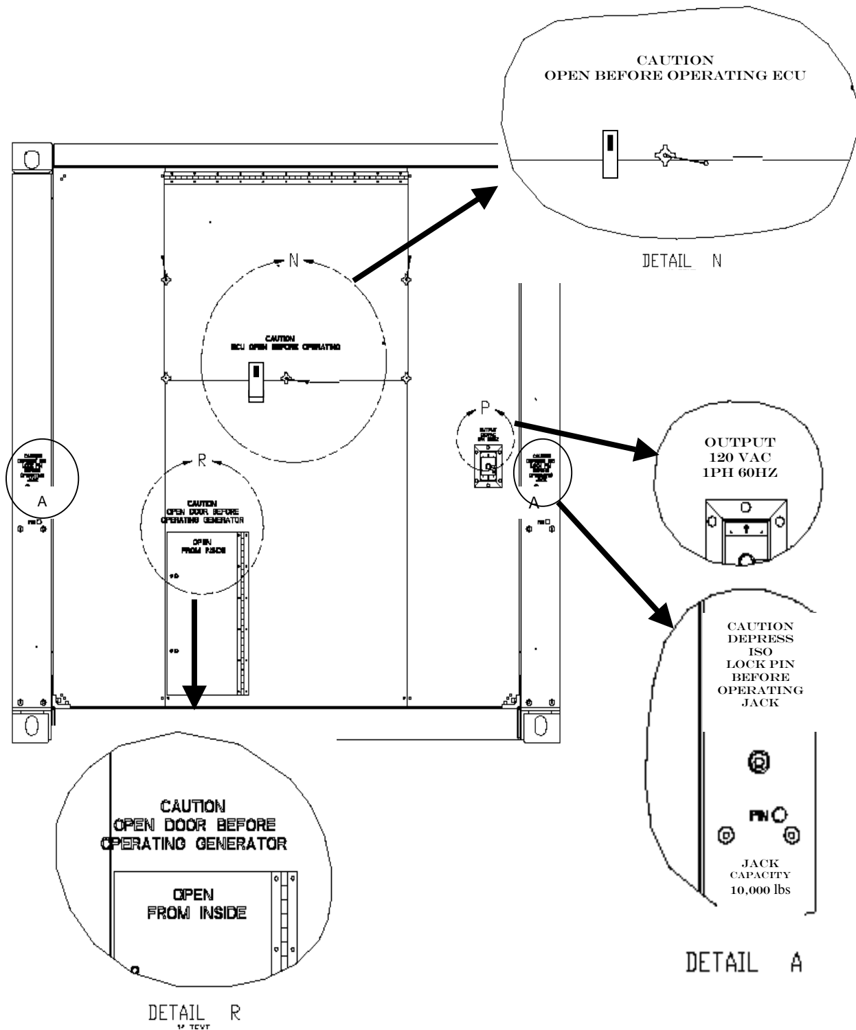
Figure 2-25. Cargo end wall stencils.
