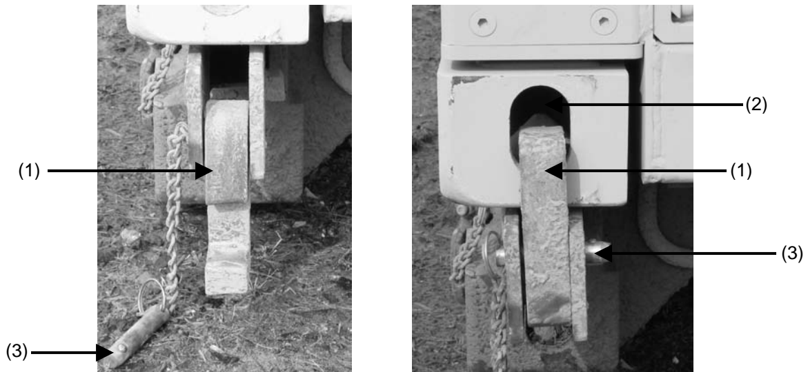
Figure 4-72. Flat rack latch.
