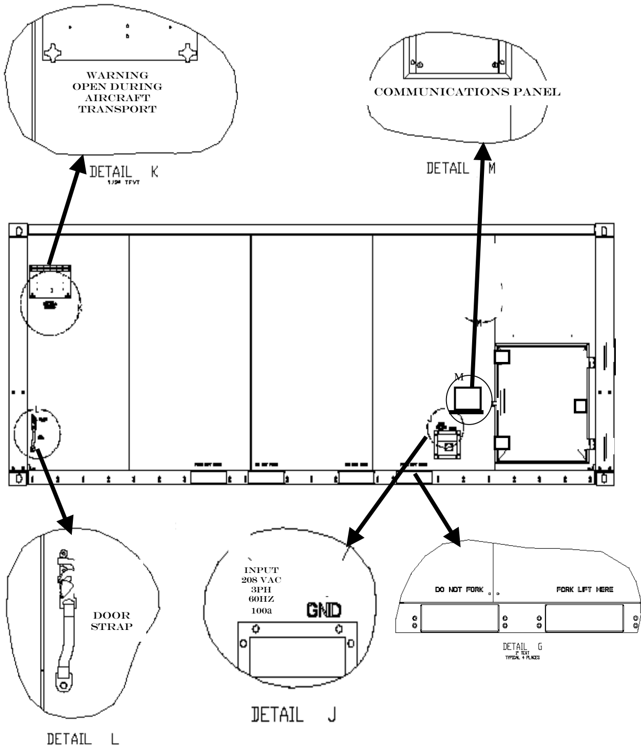
Figure 2-22. RH sidewall stencils.
