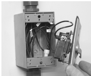
Figure 4-47. Switch pulled out of switch box.
