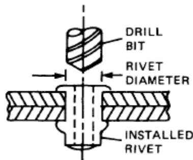
Figure 4-50. Illustration of installed rivet.
