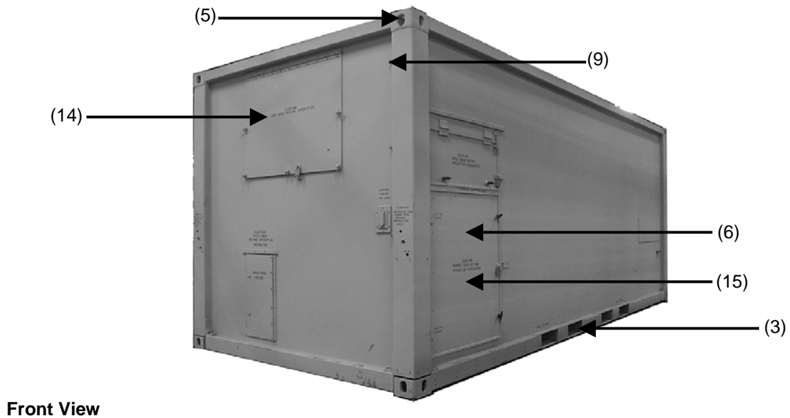
Figure 2-2. Full external view of SATS
