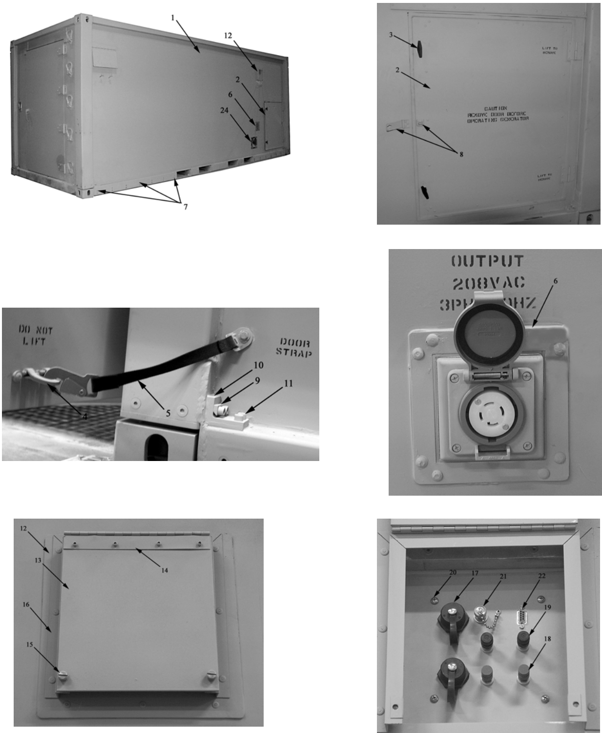
Figure 5-6. Group 0401, Right-hand Sidewall (Outside) (Sheet 1 of 2)
