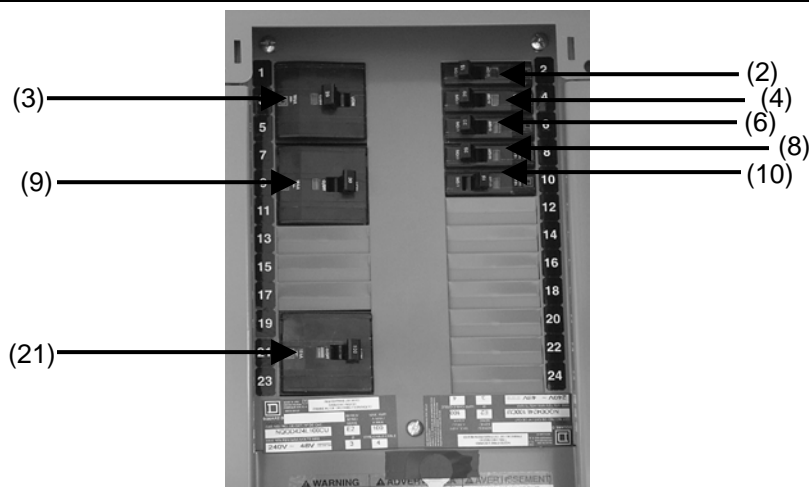
Figure 2-3. Circuit Breaker Panel
