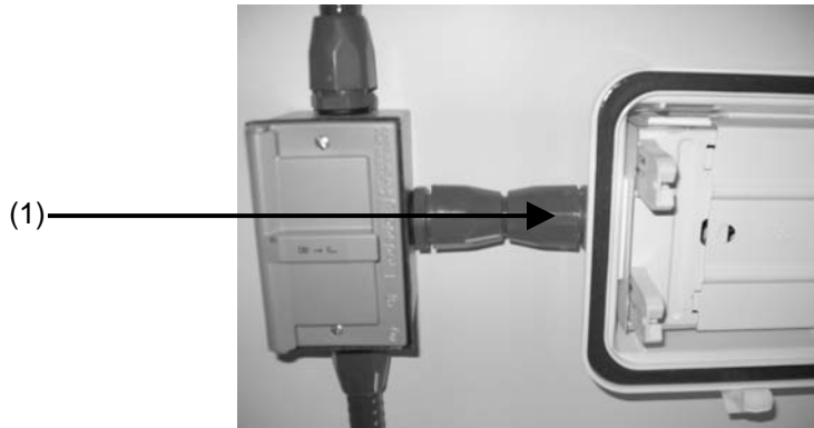
Figure 4-42. Conduit attached to ceiling light fixture.
