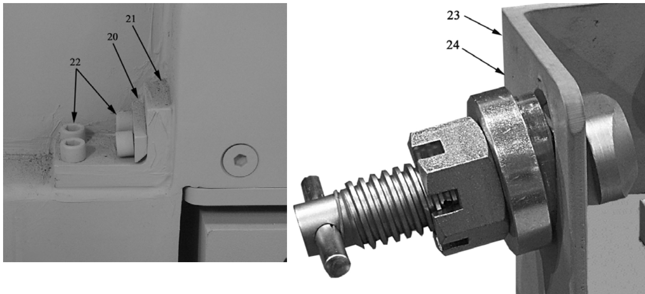
Figure 5-4. Group 0201, Outside Personnel End Wall (Sheet 3 of 3)
