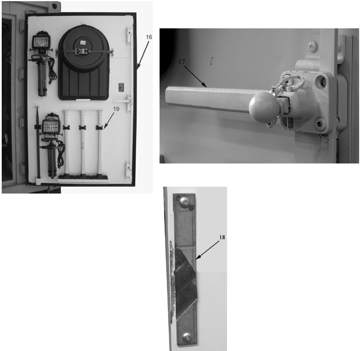
Figure 5-4. Group 0201, Outside Personnel End Wall (Sheet 2 of 3)
