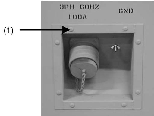
Figure 4-35. External view of Power Input Receptacle.
