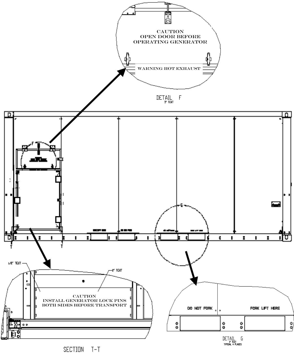
Figure 2-23. LH sidewall stencils.
