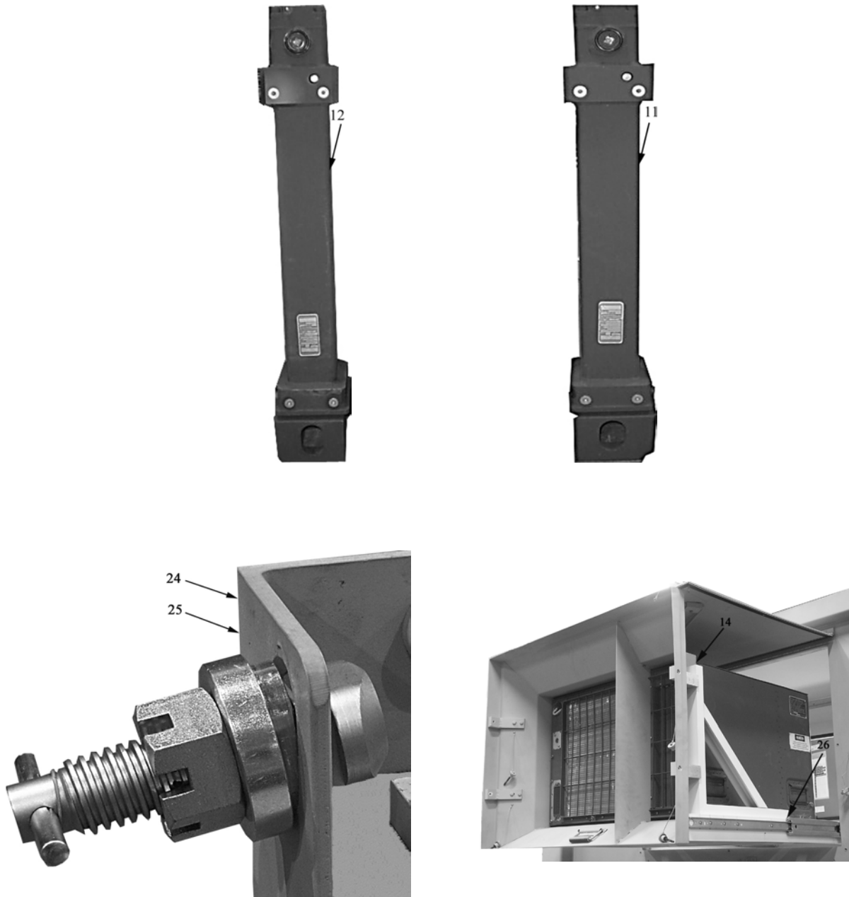
Figure 5-3. Group 0101, Environmental Control Unit, End Wall (Sheet 2 of 2)
