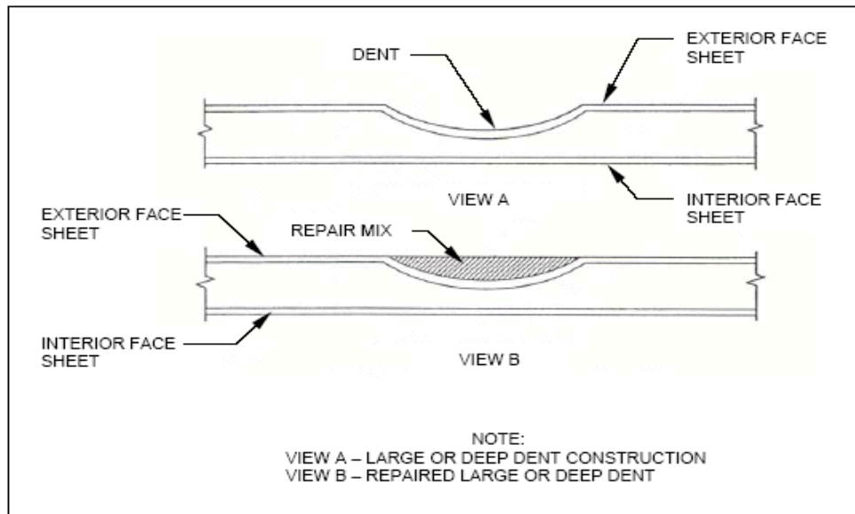
Figure 4-57. Typical Dents or Depressions
