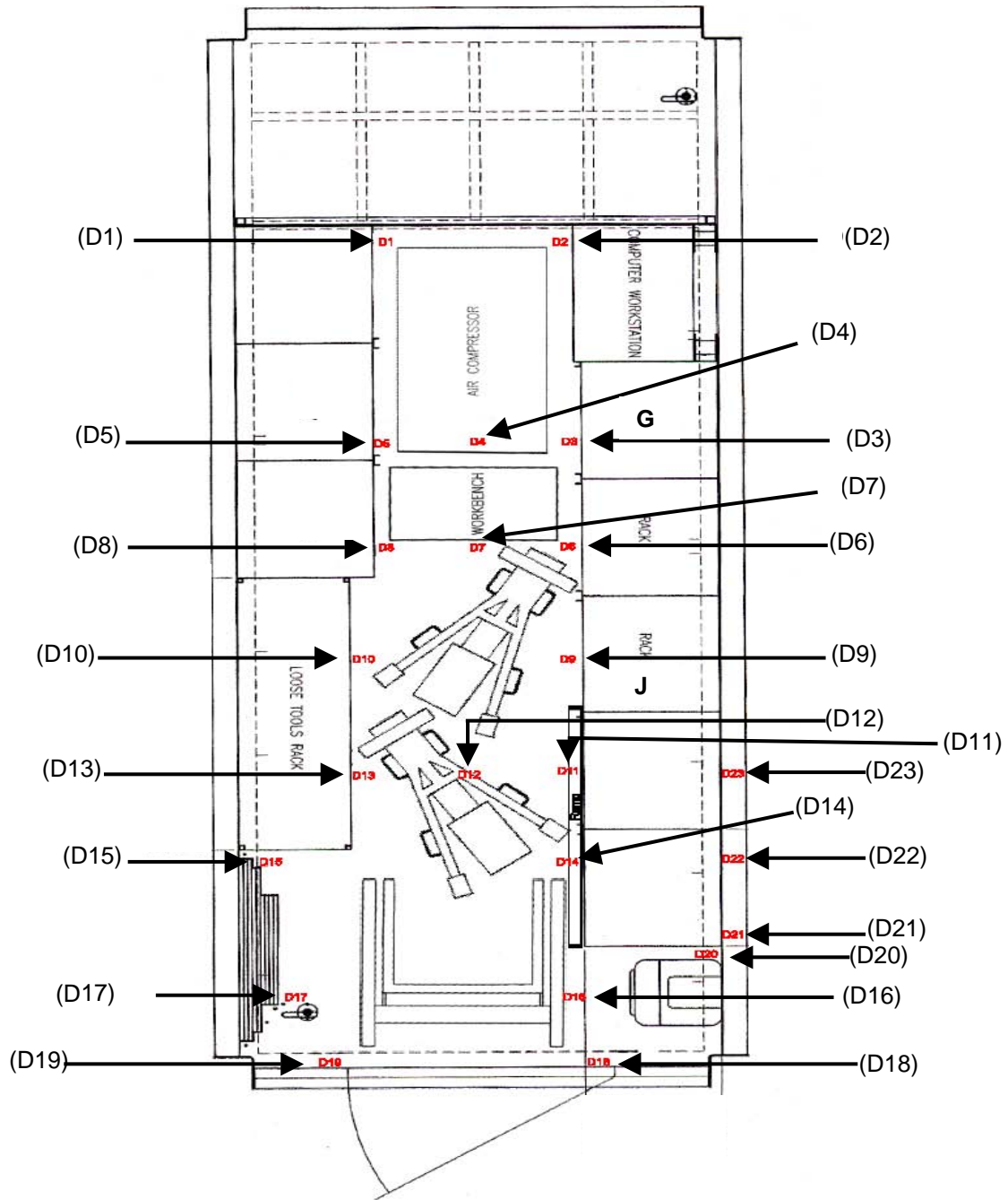
Figure 2-19. Layout of D rings in SATS.
